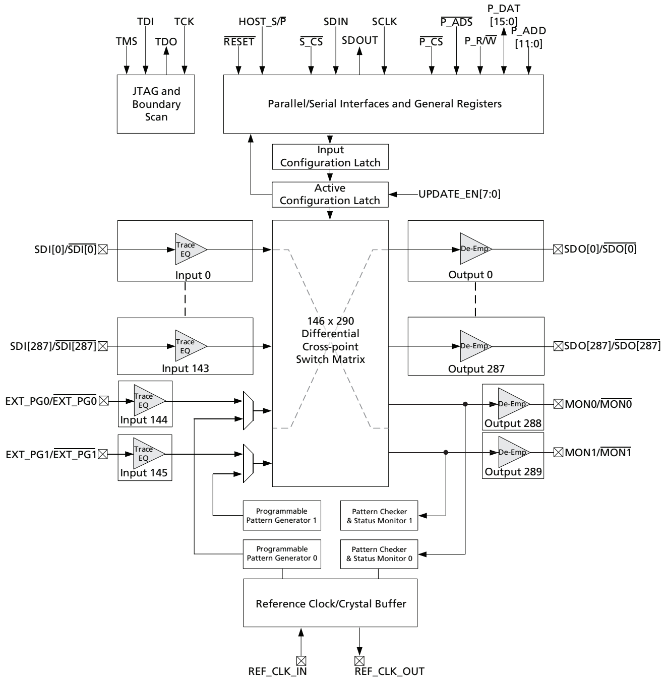
GX3190 Functional Block Diagram
