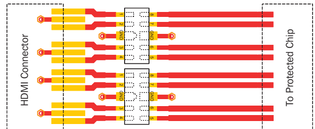
Semtech's RClamp0524P flow-through layout simplifies PCB Design
