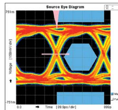
Eye Pattern Result (2.25Gbps)
