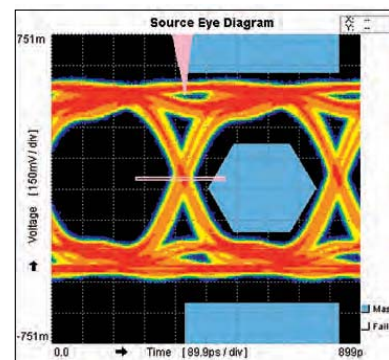
Eye Pattern Result (2.25Gbps)
