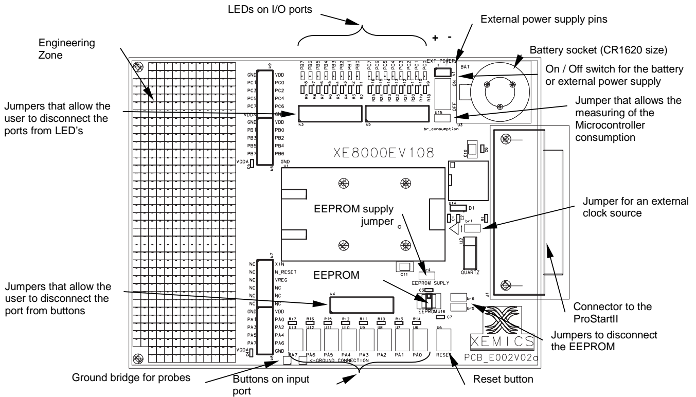
Figure 2 : Board elements
