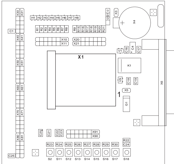
Figure 2 : XE8000EV104 implantation map
