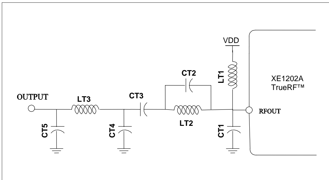
Figure 16: Transmitter output network
