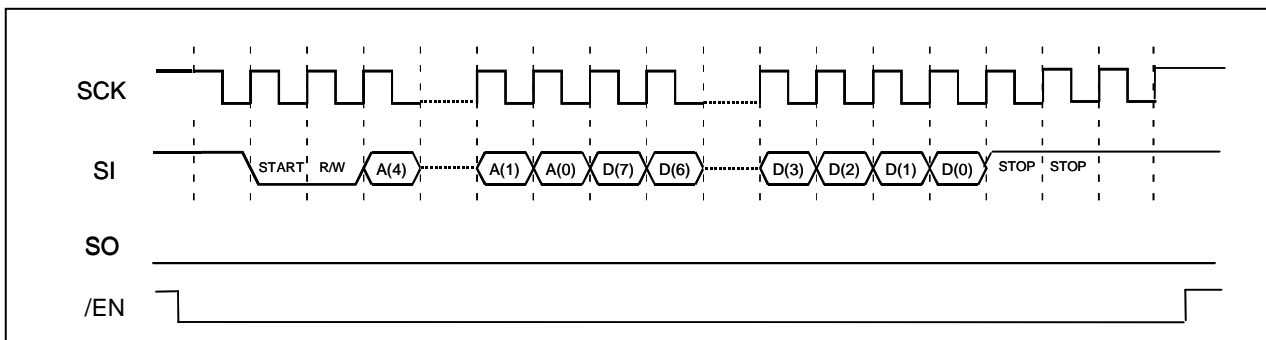
Figure 7: Write sequence into configuration register
