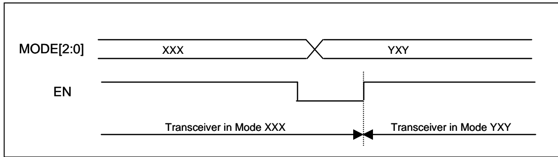
Figure 9: Switching mode sequence
