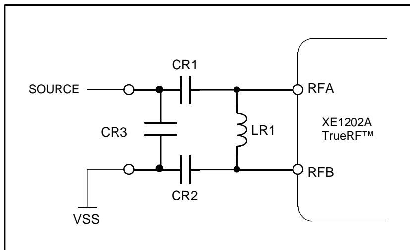
Figure 13: Receiver matching network
