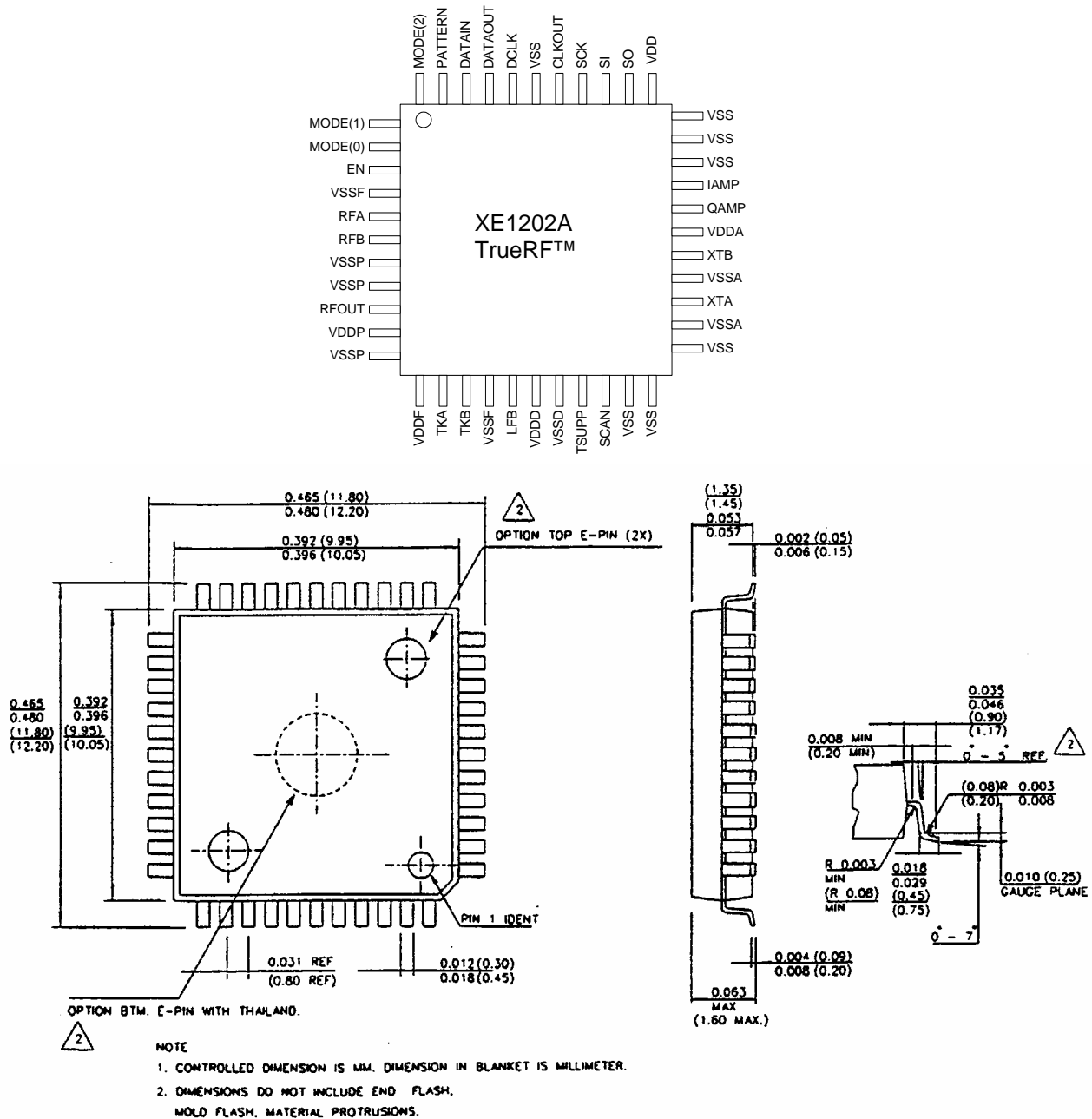
Figure 18: Package pinning and dimensions
