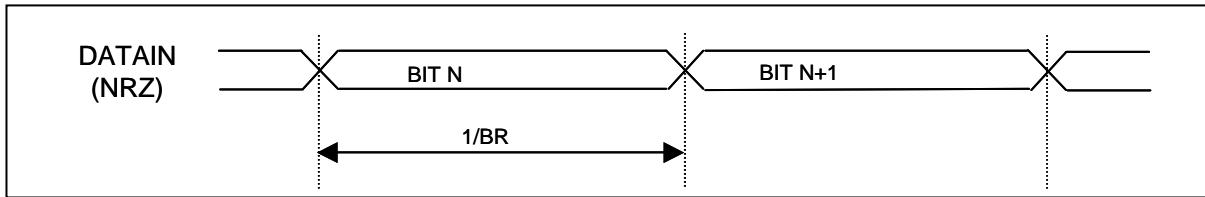
Figure 10: DATAIN timing
