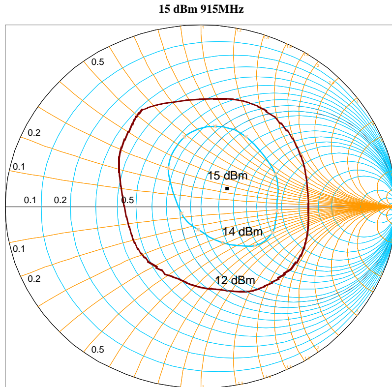
Figure 15: Output power versus load impedance at 915 MHz
