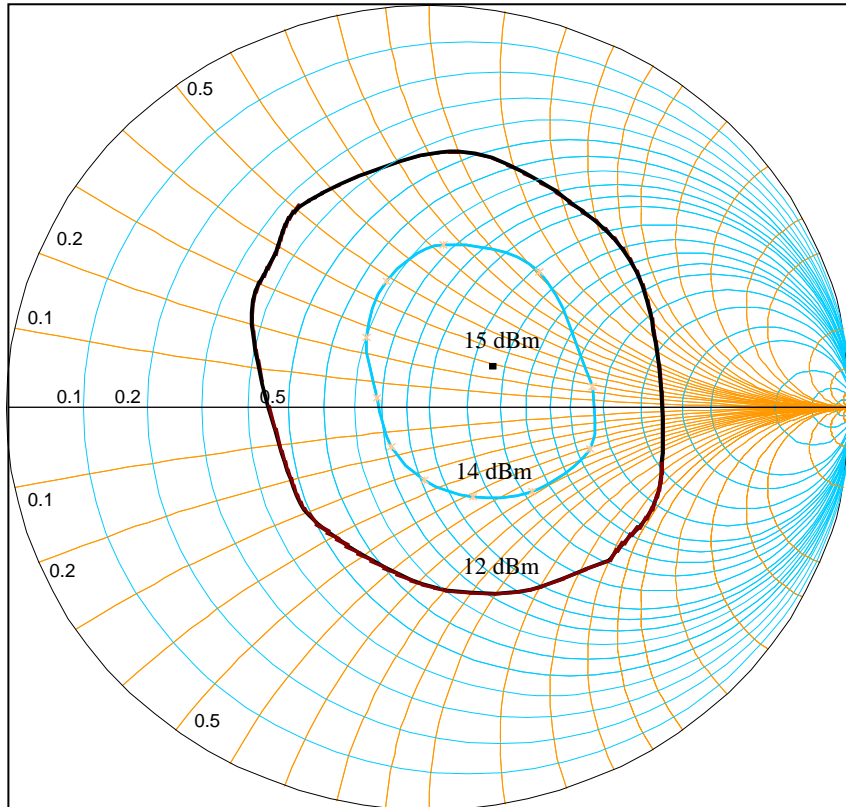
Figure 14: Output power versus load impedance at 869 MHz
