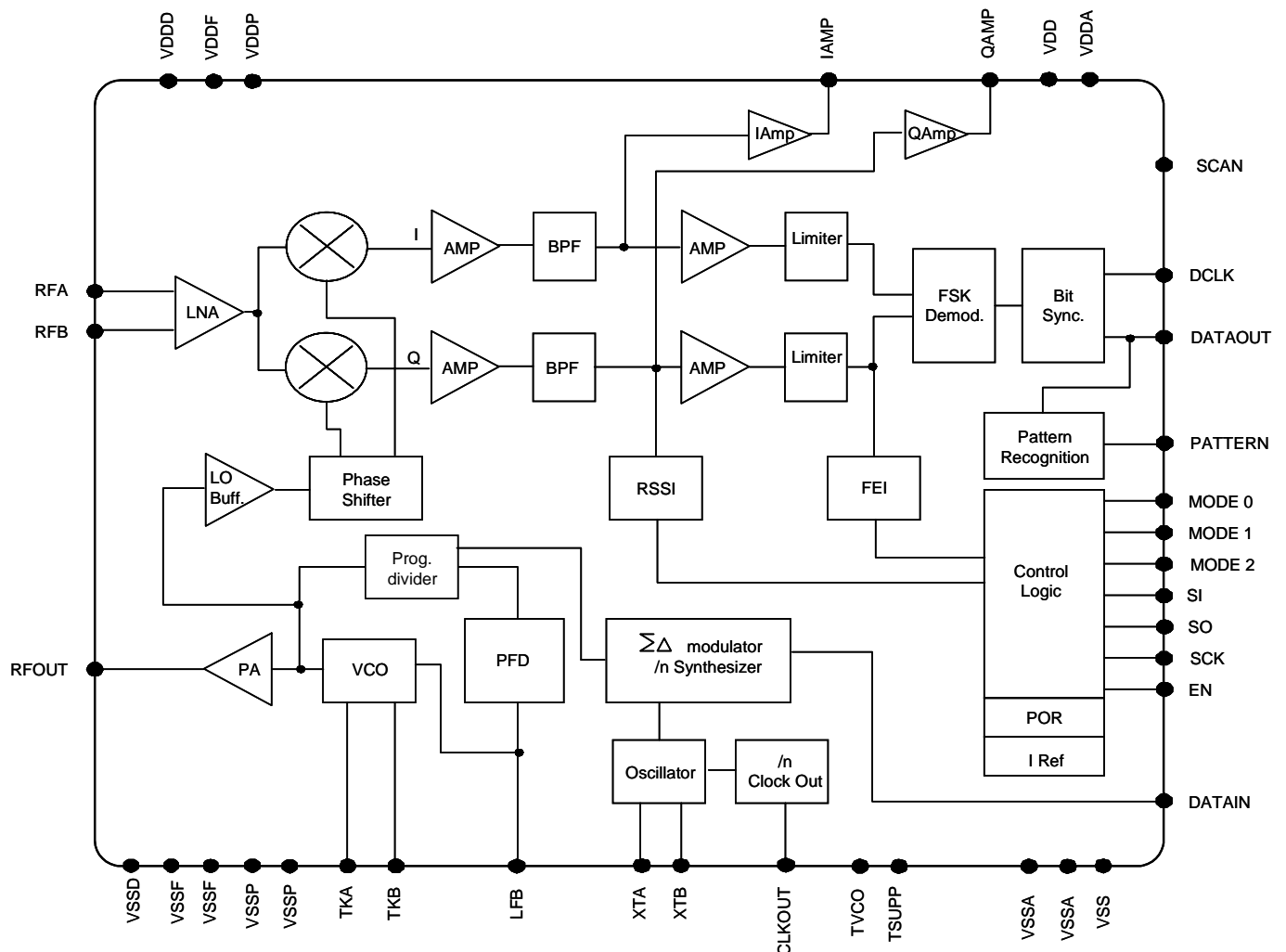
Figure 1: XE1202A TrueRF™ block diagram
