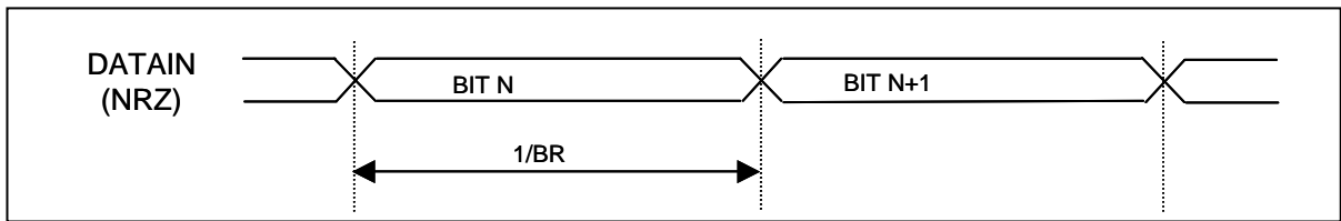
Figure 10: DATAIN timing
