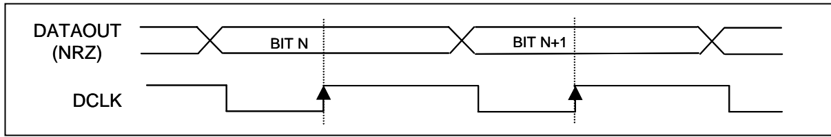
Figure 11: DATAOUT timing
