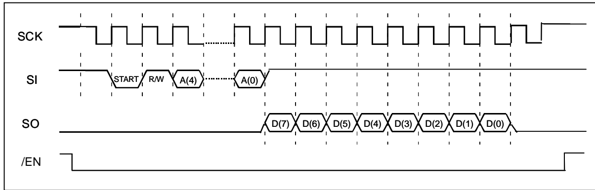
Figure 8: Read sequence into configuration register
