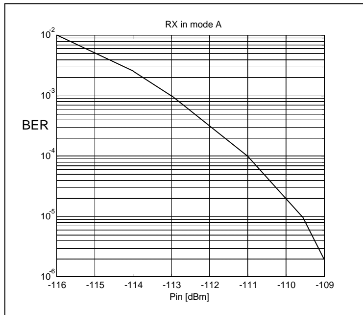
Figure 2: BER versus Rx input power with BR=4.8 kbit/s, Df=5 kHz, BW=10 kHz
