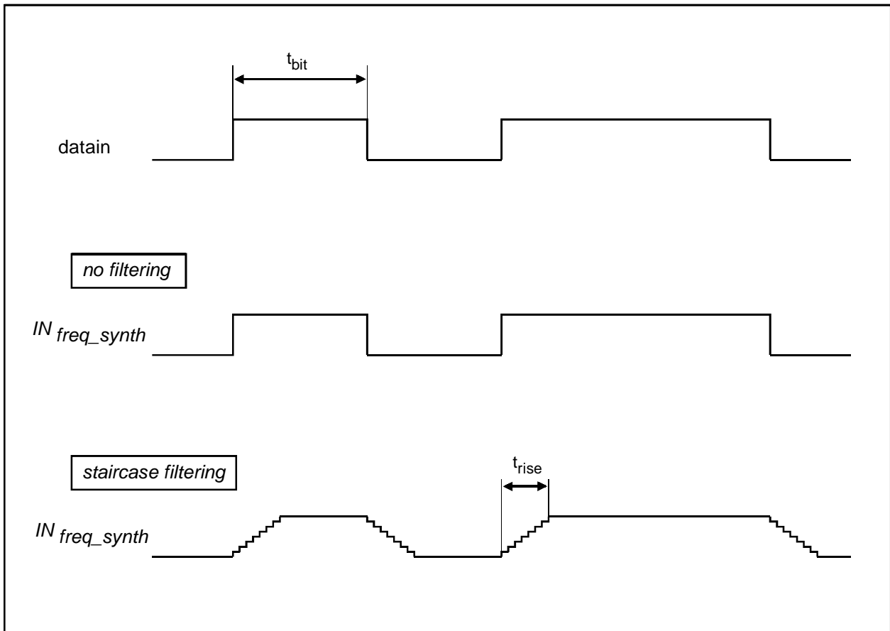
Figure 6: Modulation without and with pre-filtering
