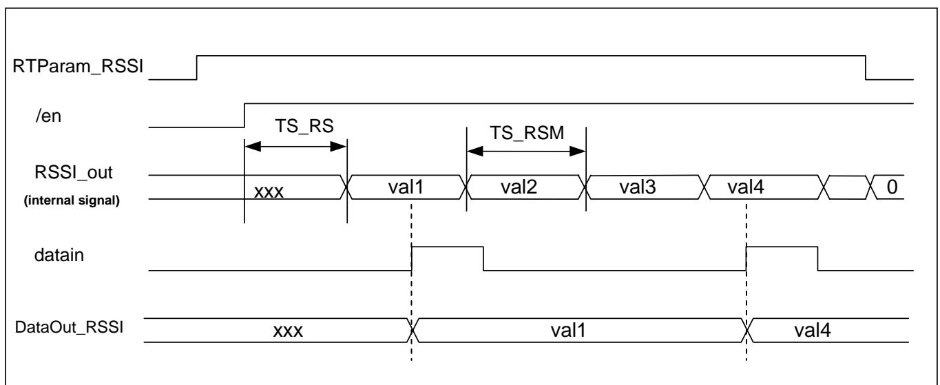
Figure 3: RSSI measurement timing diagram
