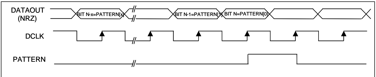
Figure 12: Pattern Recognition timing
