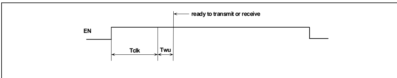
Figure 5: timing diagram for chip wake-up (from cold start)
