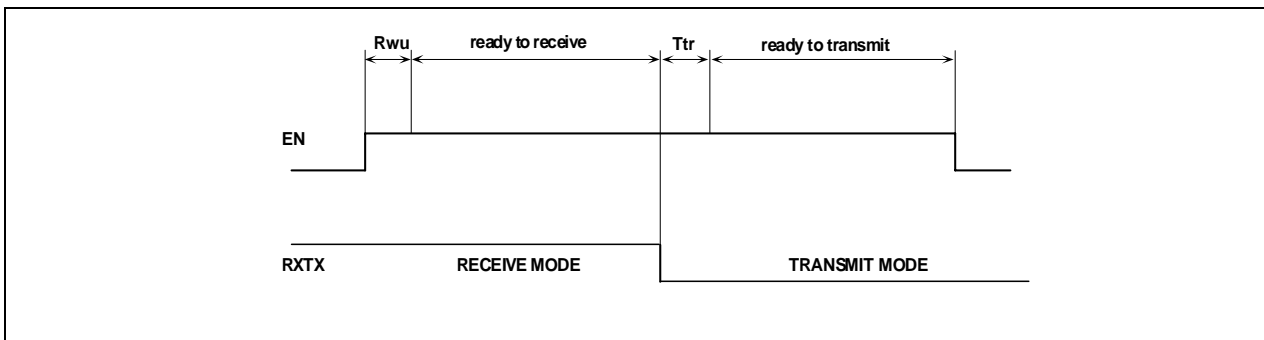
Figure 4: timing diagram for RXTX and EN control pins
