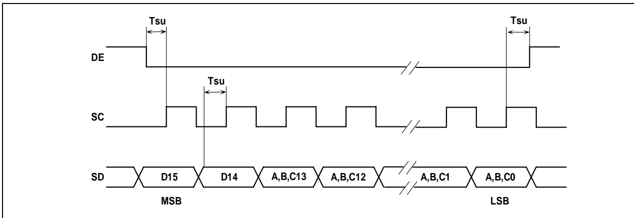
Figure 3: timing diagram for 3-wire bus
