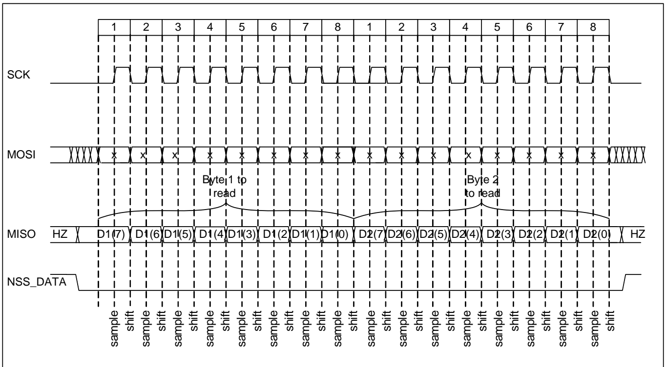
Figure 4: Reading 2 bytes in receive mode.
