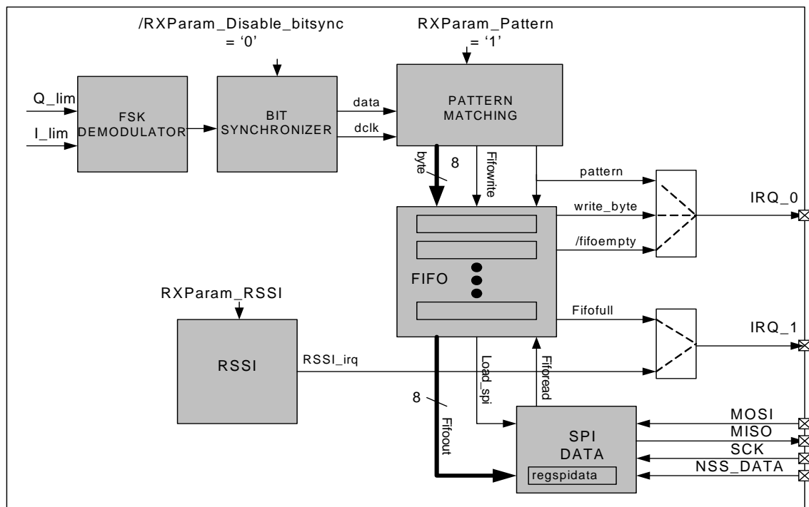
Figure 1: Receiver chain in buffered mode
