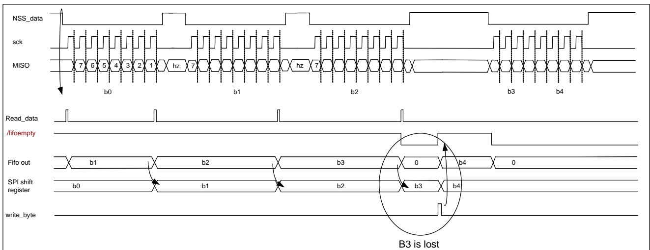
Figure 7: Losses of data
