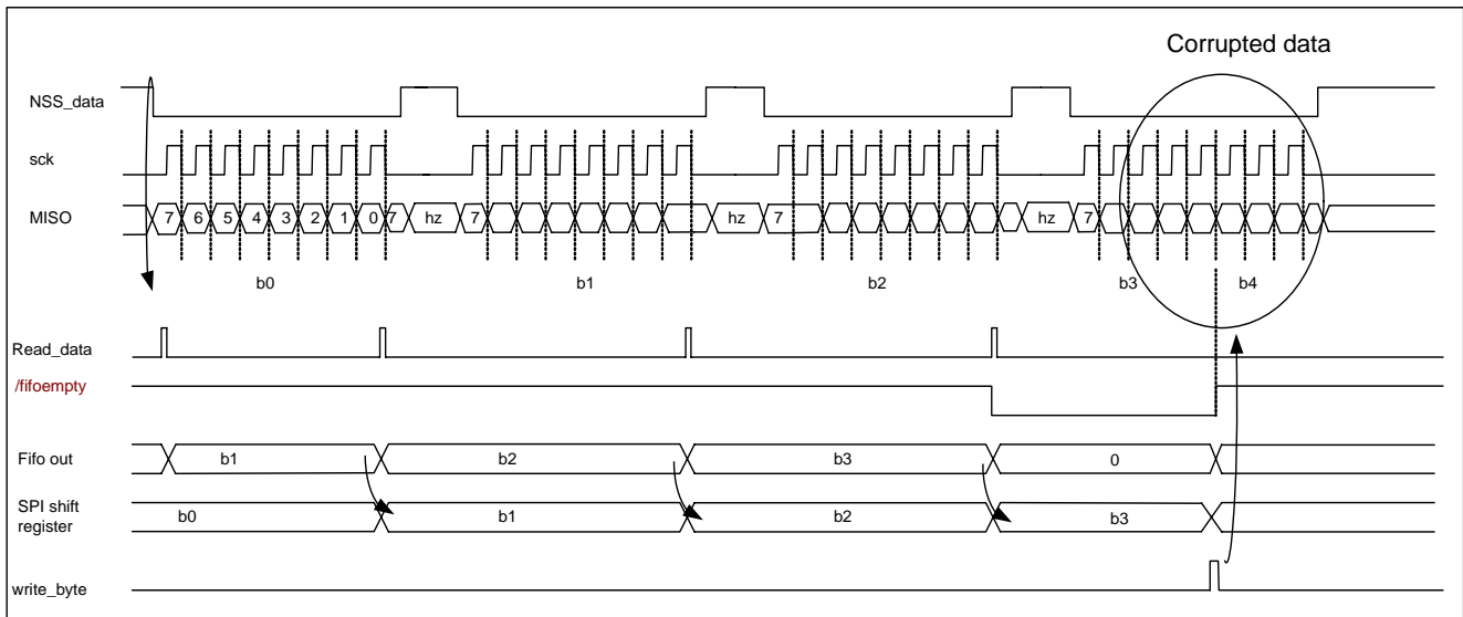
Figure 6: Corruptions of data
