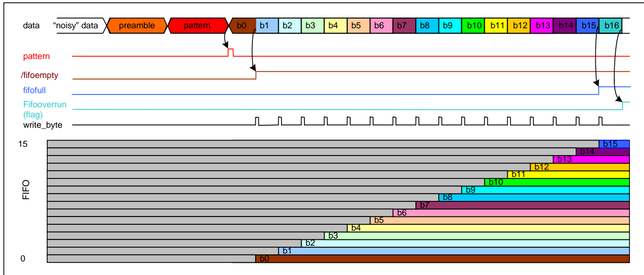
Figure 2: Standard FIFO filling
