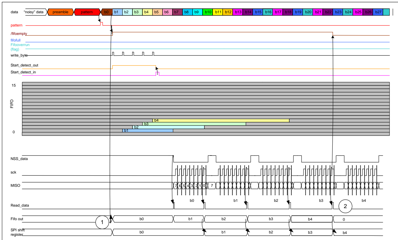
Figure 5: Standard RX timing
