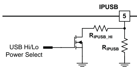
Figure 6 — External programming of arbitrary USB high power and low power charge currents.
