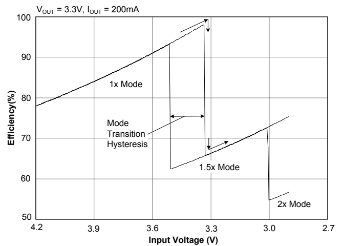
Efficiency — 200mA
