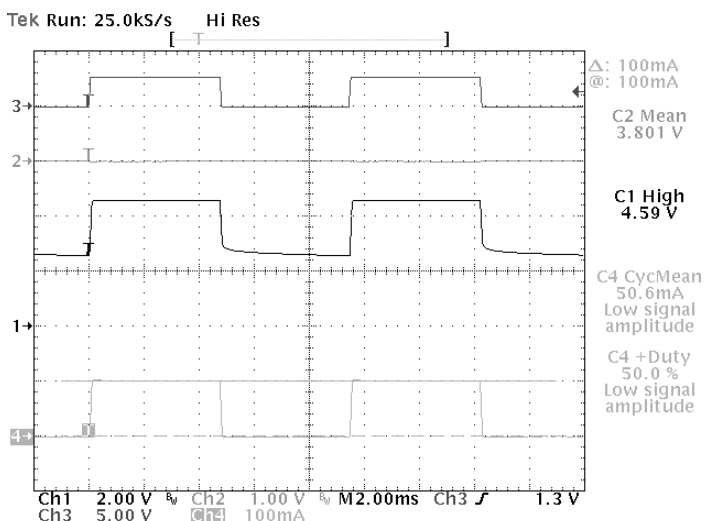
Recommended Minimum 100Hz PWM
