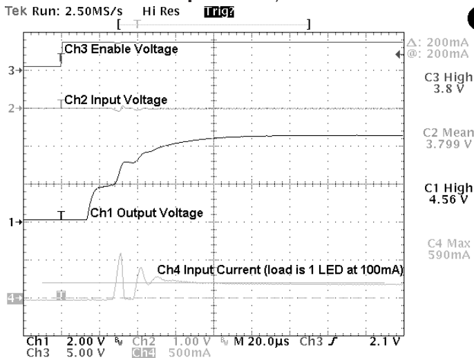
Start Up for 4.5V, 100mA
