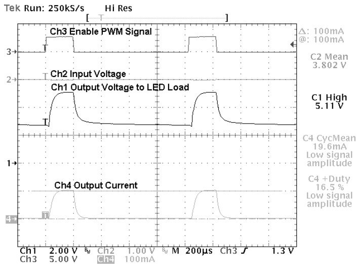
Recommended Minimum High Pulse Width
