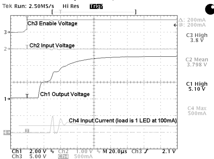
Start Up for 5.0V, 100mA
