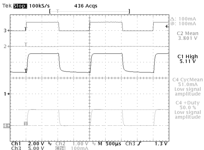
Recommended Maximum 500Hz PWM
