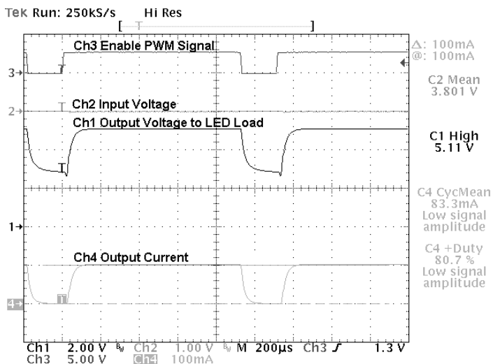
Recommended Minimum Low Pulse Width
