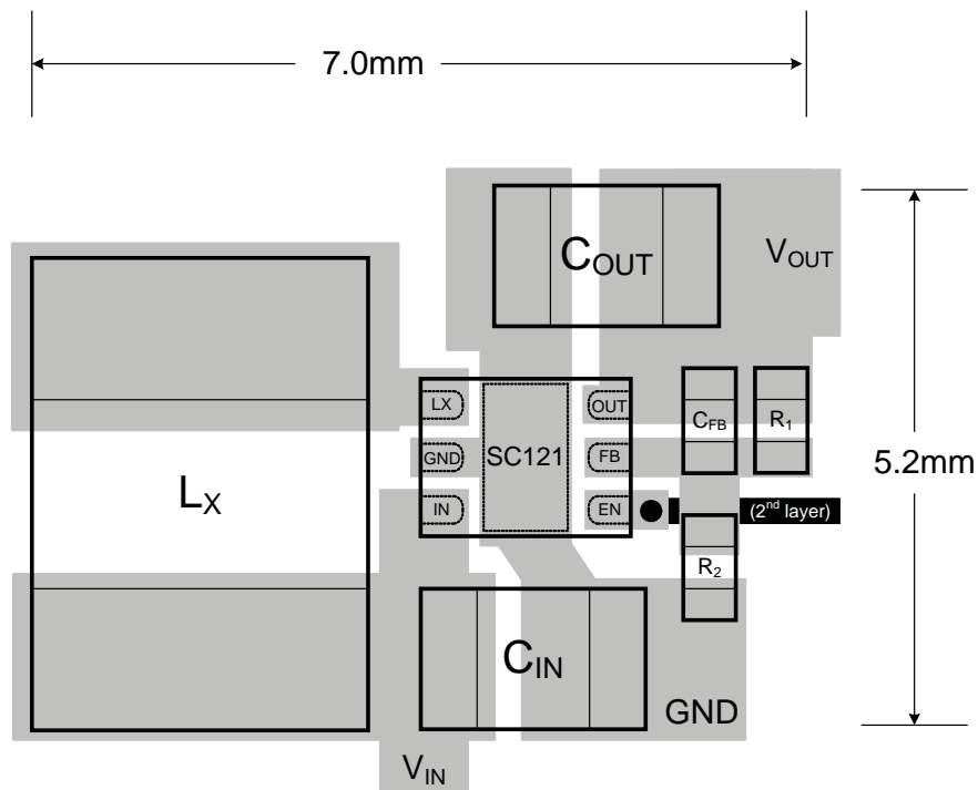
Figure 4 — Layout Drawing
