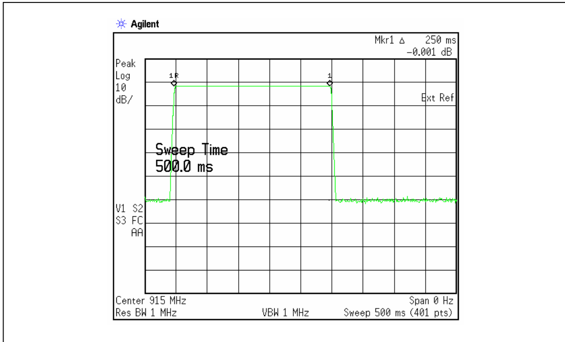
Figure 4: Measurement of Hopping Channel Dwell Time
