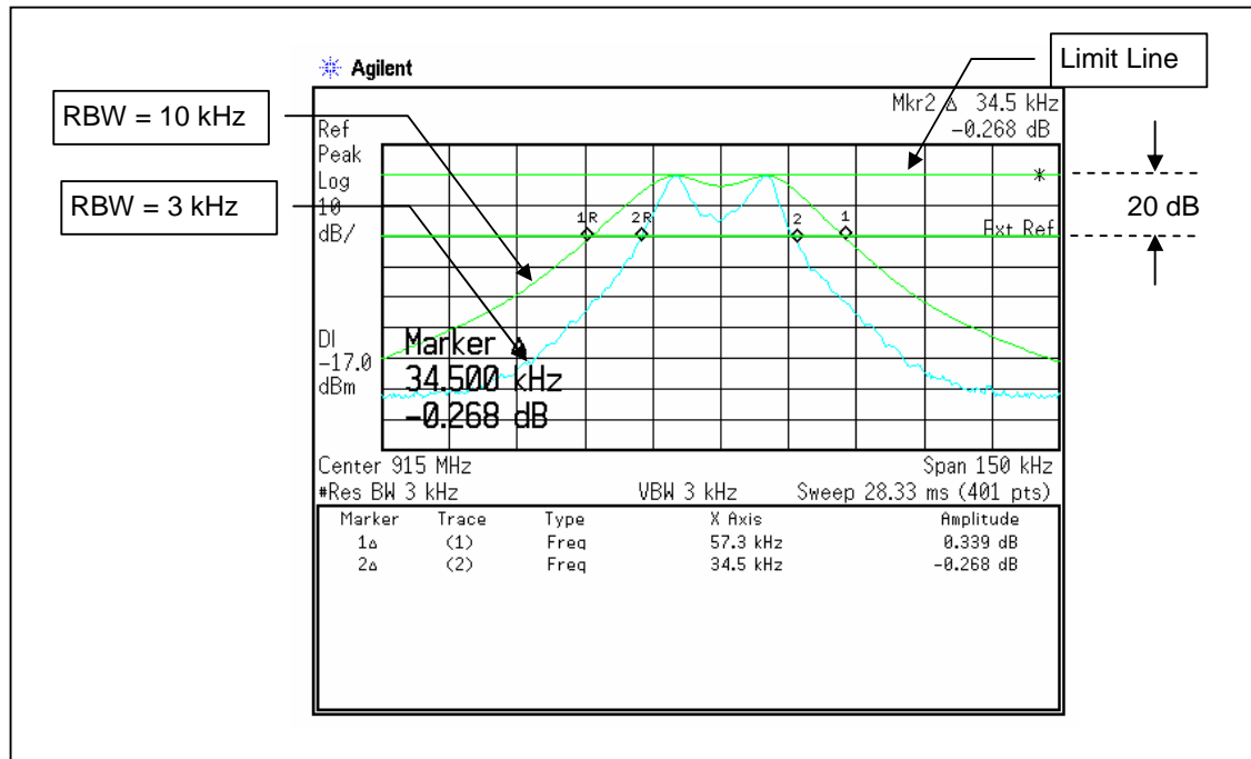
Figure 2: Measurement of 20 dB Bandwidth
