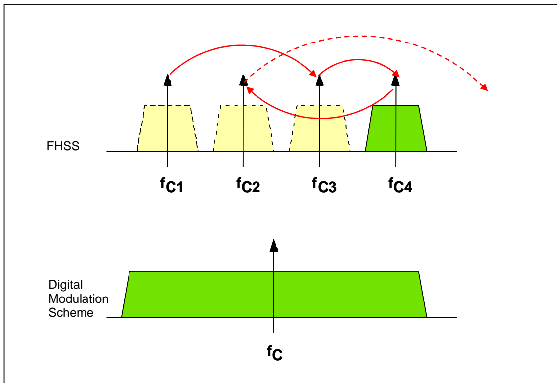
Figure 1: FHSS and Digital Modulation Scheme Spectrums
