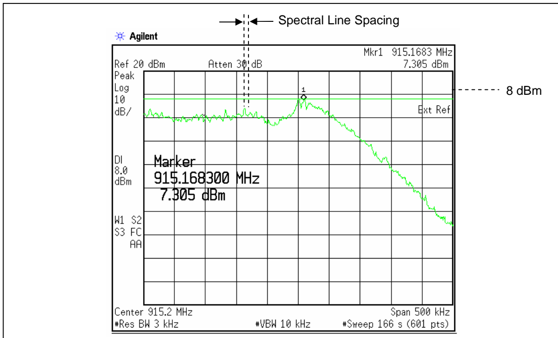
Figure 7: Measurement of Peak Spectrum Density
