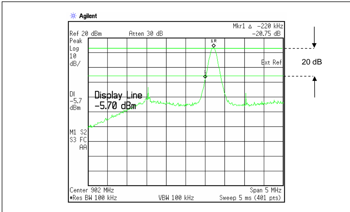
Figure 5: Transient Band Edge Conducted Emissions Measurement
