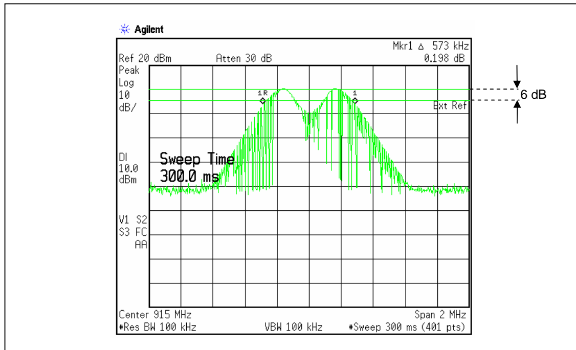
Figure 6: Measurement of Signal Bandwidth
