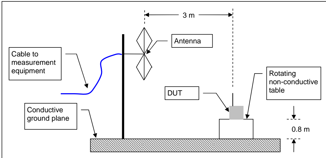
Figure 8: 3 Meter Test Site
