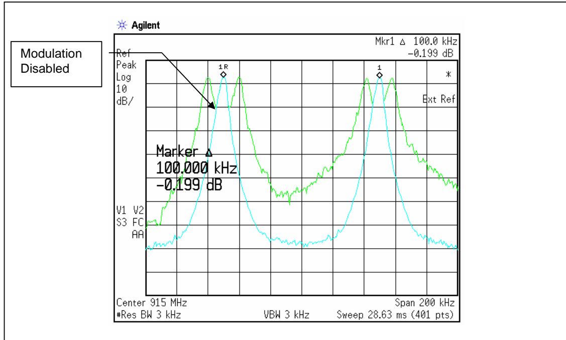
Figure 3: Measurement of Carrier Frequency Separation
