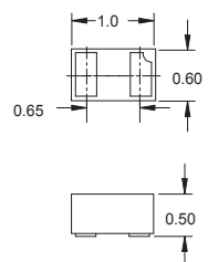
SLP1006P2
