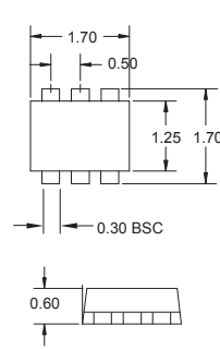
SLP1510N6
