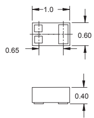
SLP1006P3T
