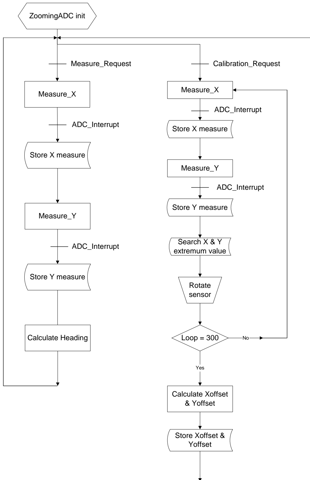
Figure 10 : Measurement Flowchart
