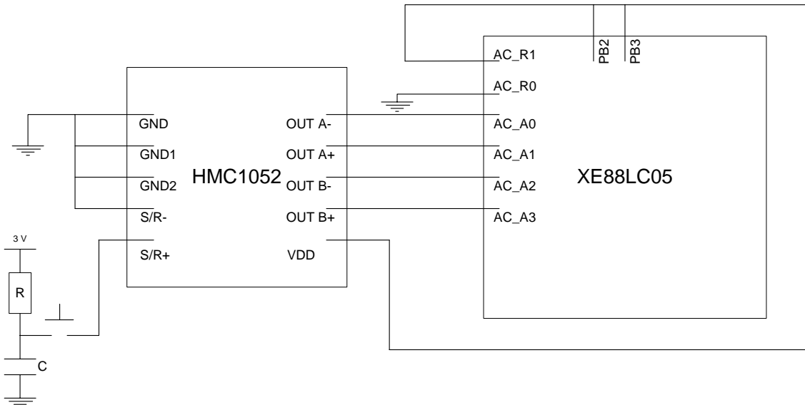
Figure 7 : HMC1052-XE8805/05A interface
