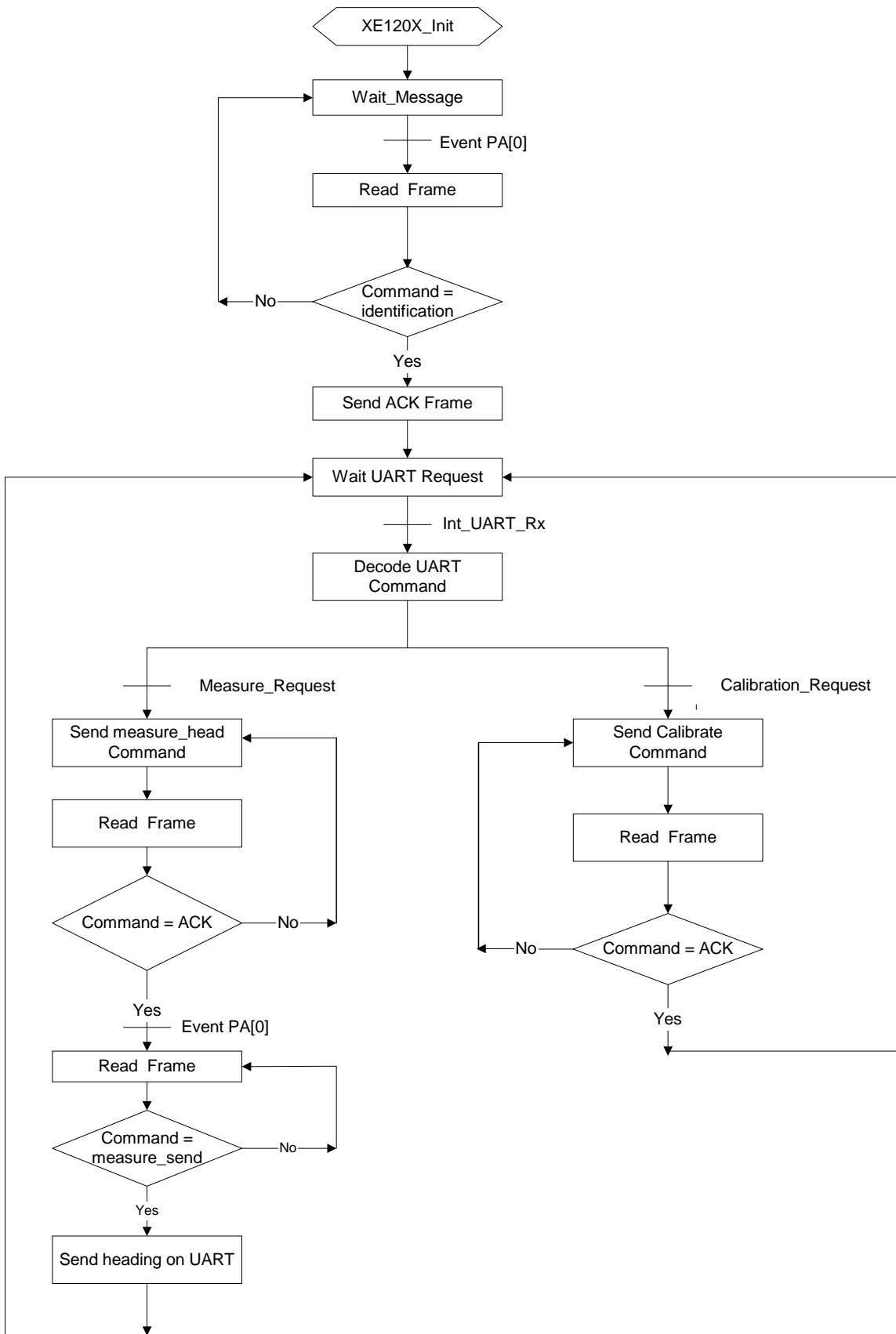
Master Flowchart
