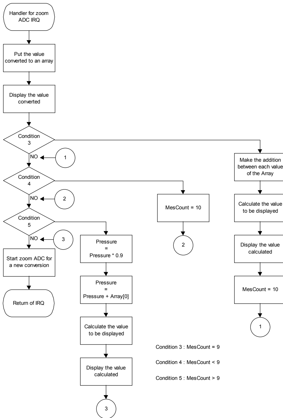
Zoom ADC Irq handler routine Figure 9
