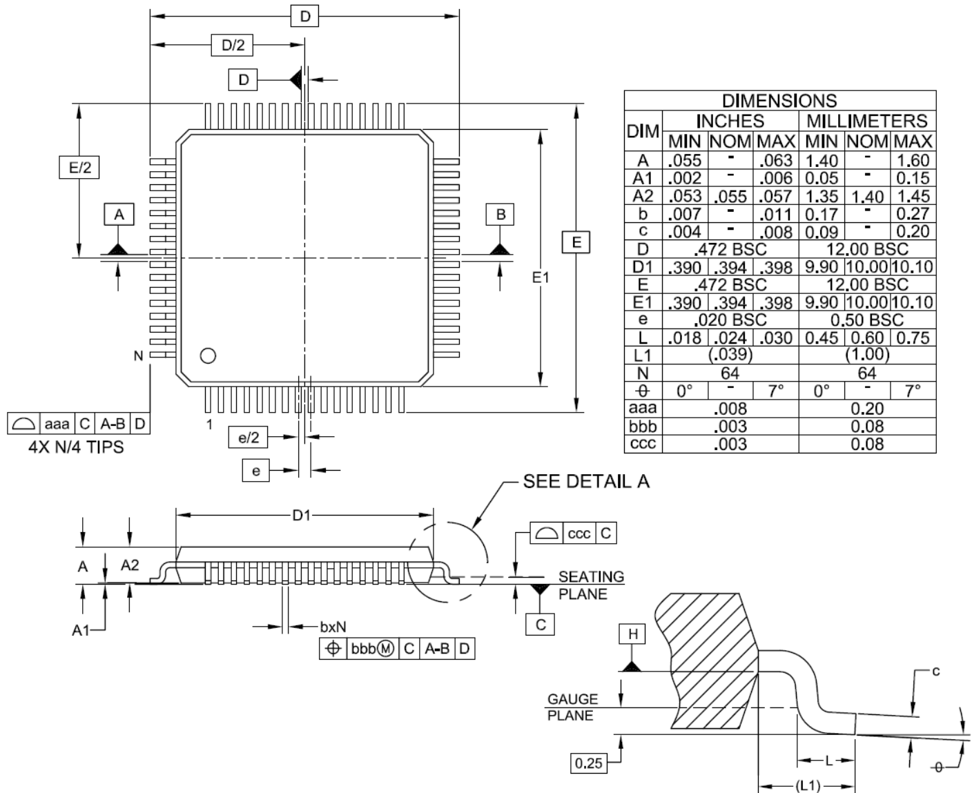
Figure 6 LQFP Package
